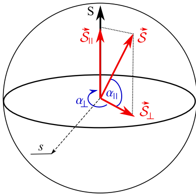
FIG. 1 (color online). Transformation from the frame of the vector \mathbf{S} to that of \vec{S} . Angles \alpha_{\parallel,\perp} define the modulus of the “transverse” component \vec{S}_\perp and its rotation around the “longitudinal” component \vec{S}_\parallel , respectively.
